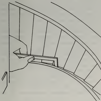
FIGURE 10-67. Measuring turbine wheel to exhaust cone clearance.
